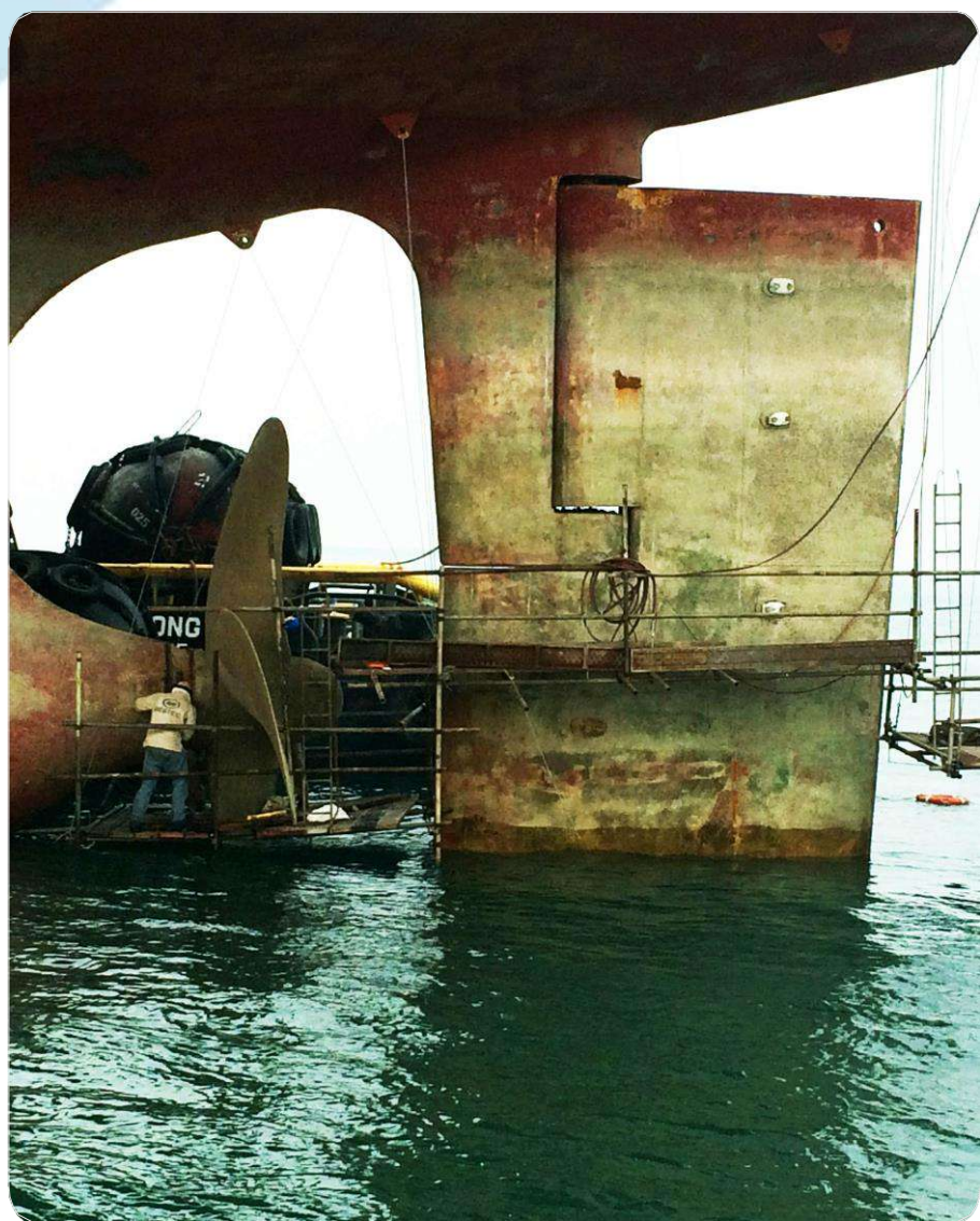
Sterntube seal renewal works
