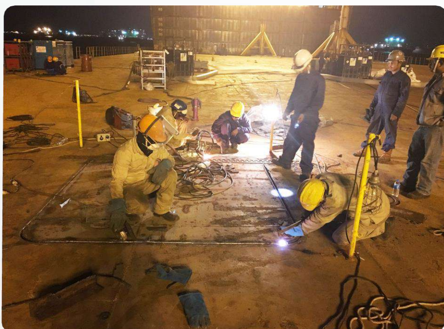
Reinstating works for heavy load transport vessel
